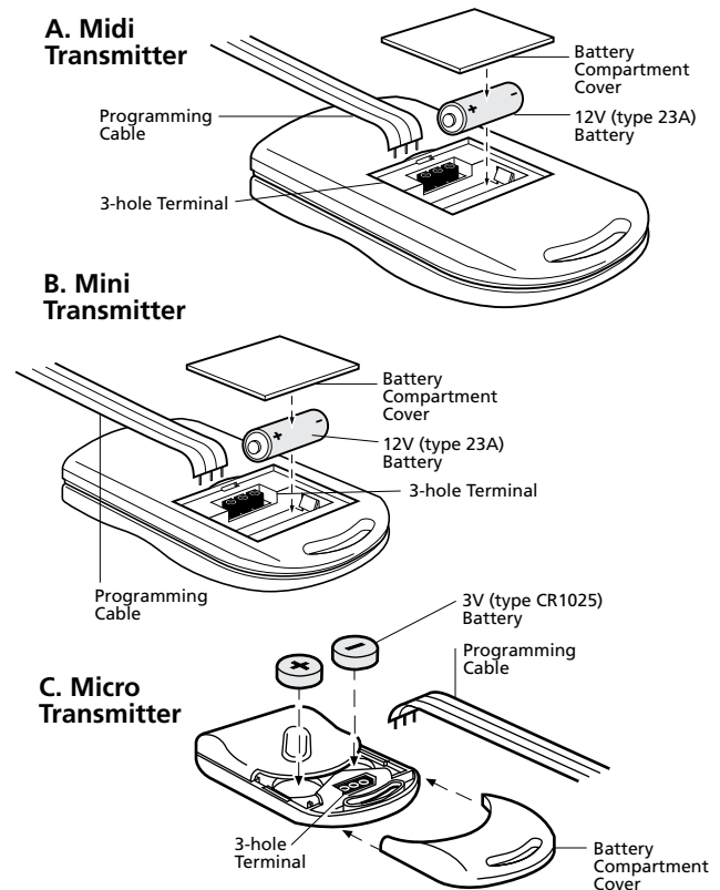
Figure 1. Battery Compartment
